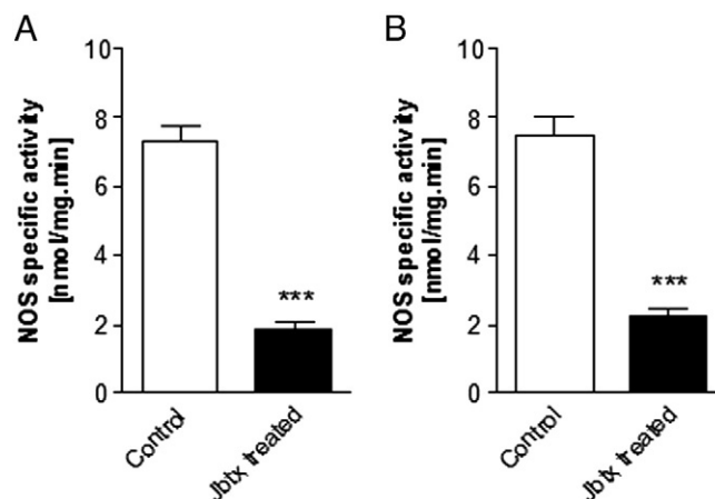
Fig. 4. Effect of Jbtx on NOS activity in T. infestans CNS. (A) Insects were injected with vehicle (control) or with the peptide (Jbtx treated, 0.1 µg/mg body weight). For each treatment, the CNS of the insects were dissected, pooled and processed for determination of the enzymatic activity as described in Section 2. Results are expressed as nmol of NO produced/mg.min and are means ± SEM (n = 4–6). *** P < 0.001, df = 8, Student t test. (B) For in vitro experiments, CNS homogenates were incubated with vehicle (control) or with 1 nM Jbtx (Jbtx treated), followed by NOS activity determination. Results are means ± SEM (n = 4). *** P < 0.001, df = 6, Student t test.
